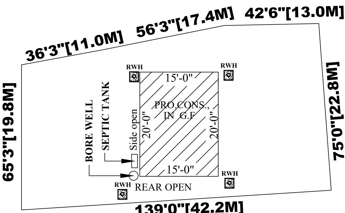
SITE PLAN
