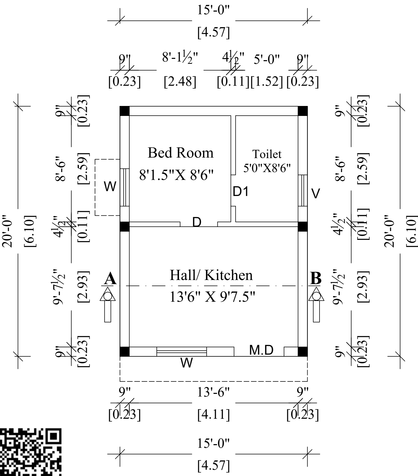
D. GROUND FLOOR PLAN
