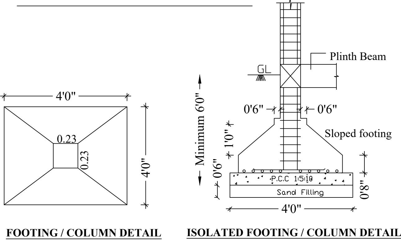
FOOTING / COLUMN DETAIL
