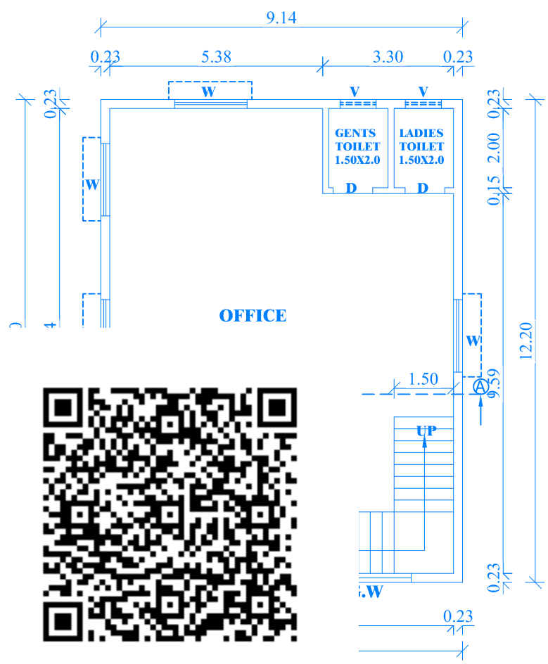
OFFICE PLAN
