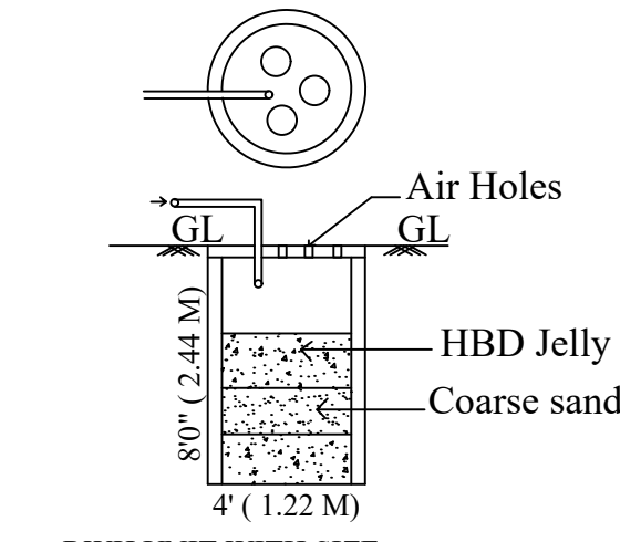
RAIN WATER HARVESTING TANK DETAIL
