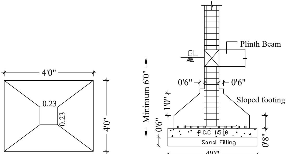
FOOTING / COLUMN DETAIL
