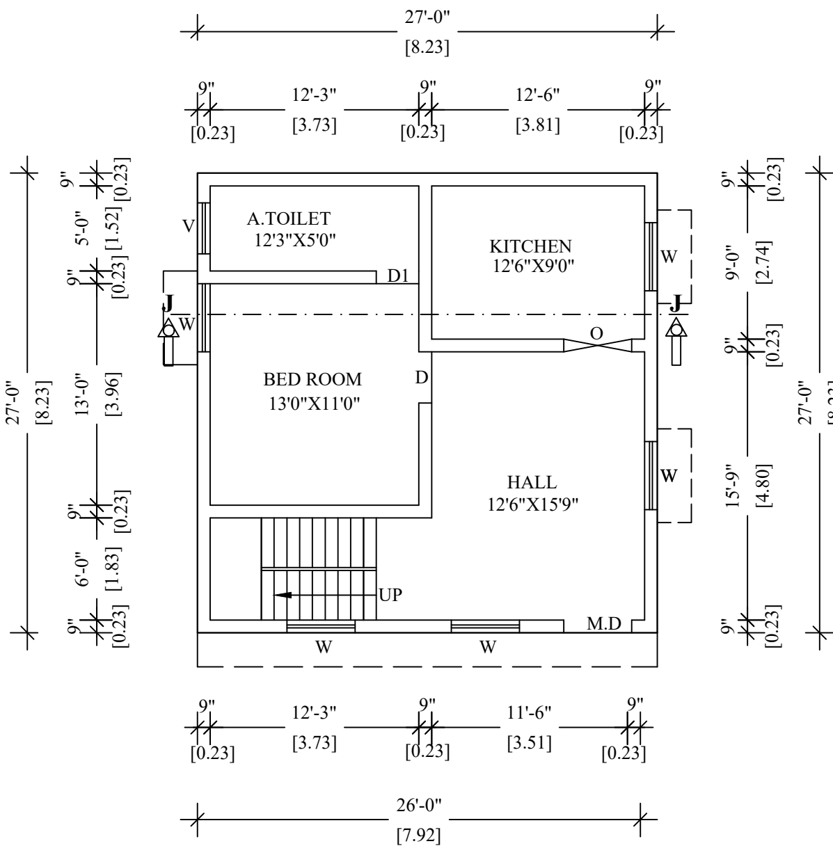
EXI. GROUND FLOOR PLAN
