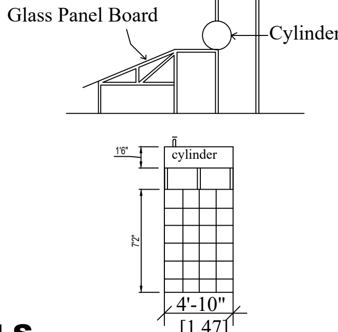
SOLAR ENERGY SYSTEM
