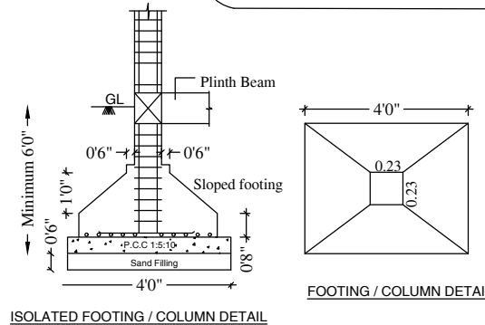
COLUMN DETAILS
