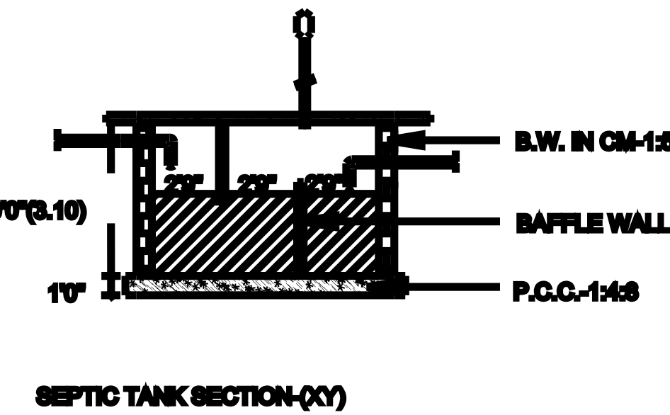
SEPTIC TANK SECTION (XY)
