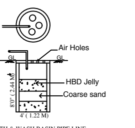
WASTE WATER RECYCLE UNIT
