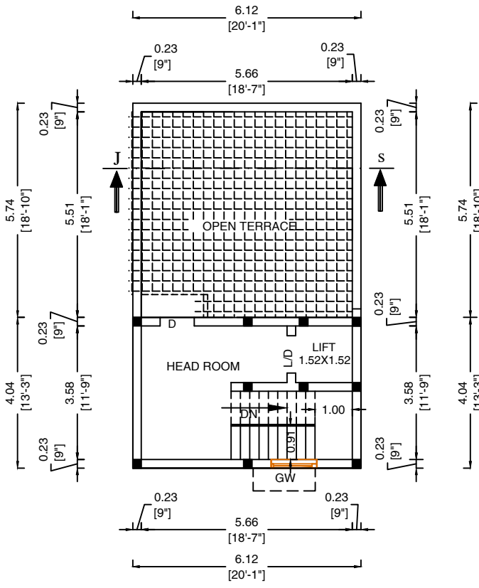
OPEN TERRACE FLOOR PLAN
