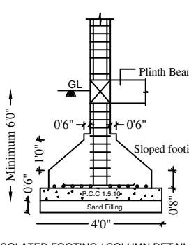
COLUMN DETAILS
