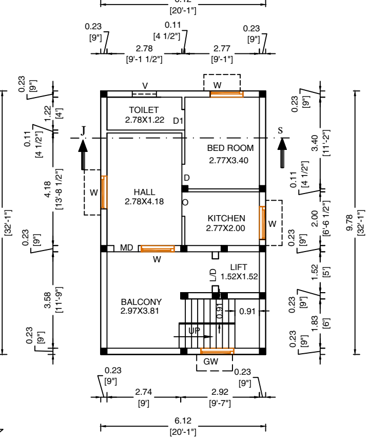
TYPICAL FLOOR PLAN (1st, 2nd FLOOR PLAN )
