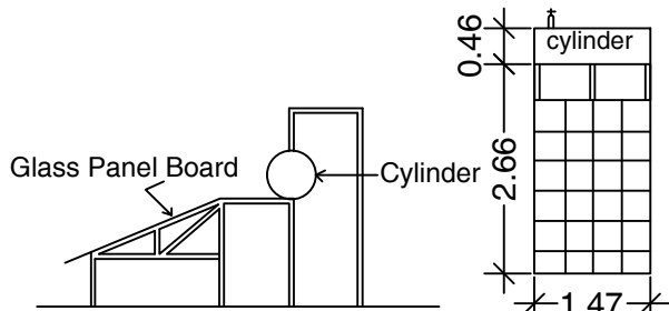
SOLAR ENERGY SYSTEM
