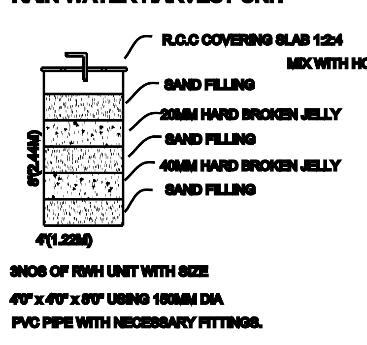
RAIN WATER HARVEST UNIT
