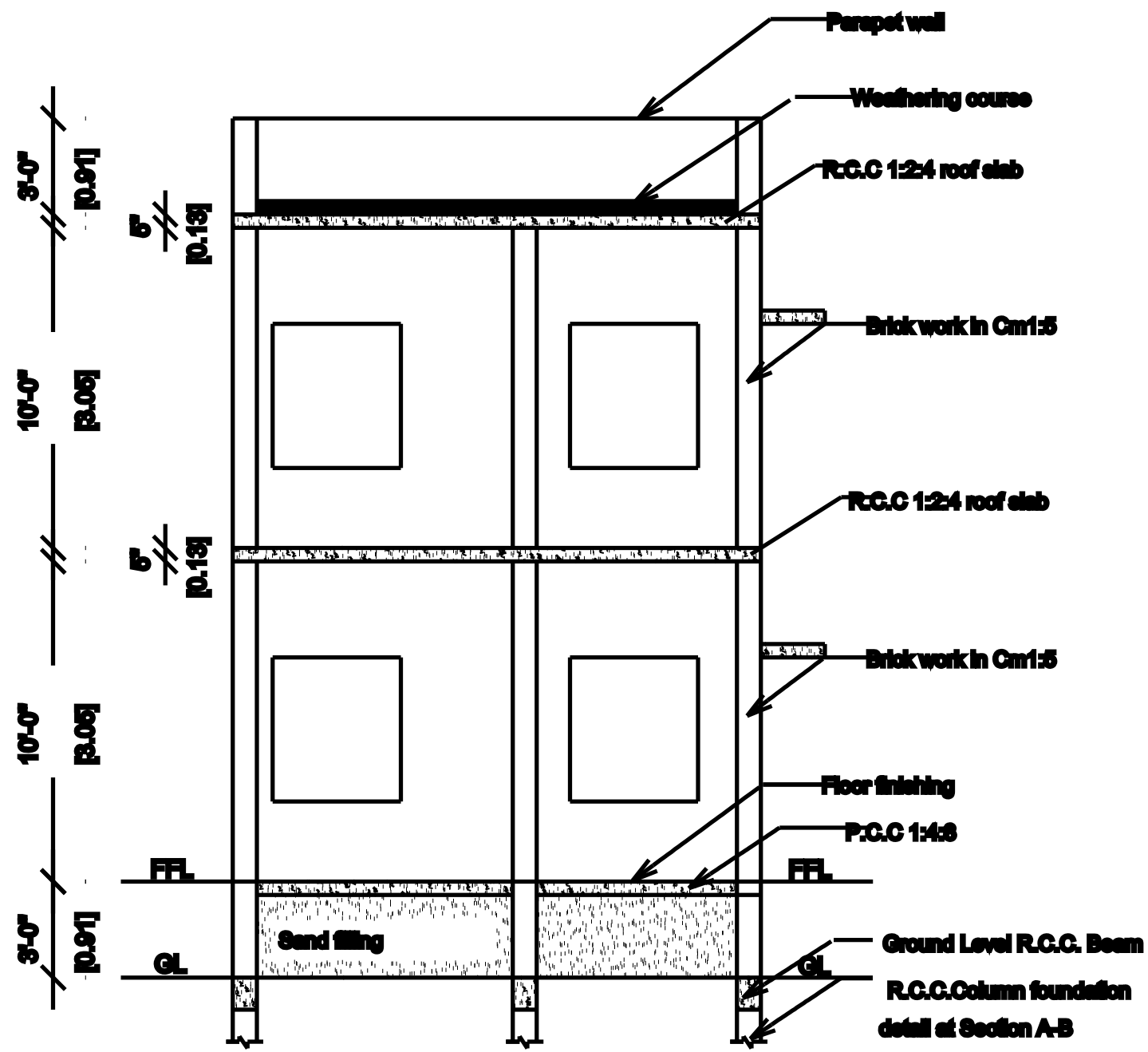
SECTION ON 'SA'
