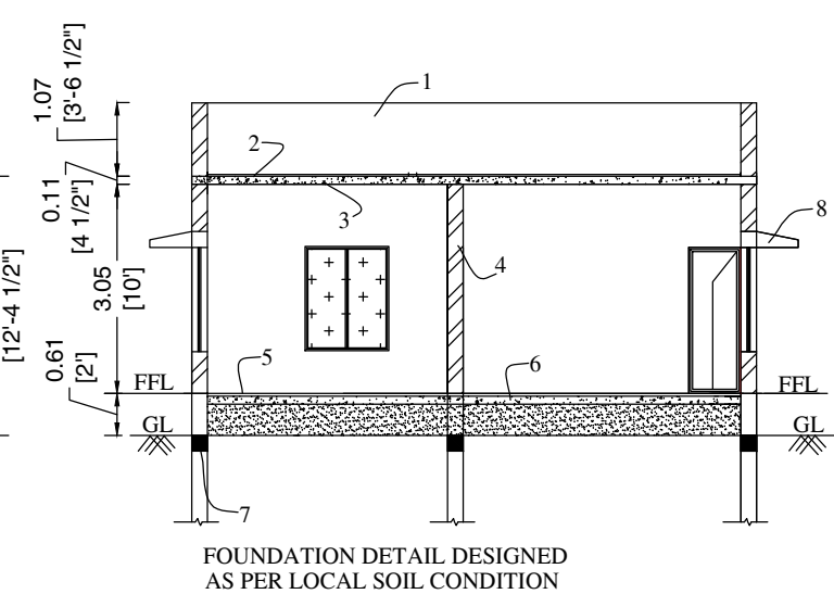
SECTION ON "JS"
