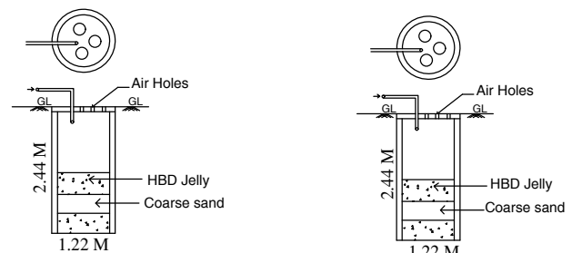
RAIN WATER HARVESTING TANK DETAIL
