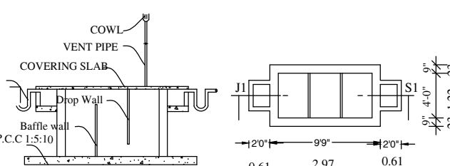
SECTION ON JS1 Using 'U' type trap 2 Nos in inlet, outlet & Vent pipe will be covered with mosquito proof net in inner side and top of the vent pipe
