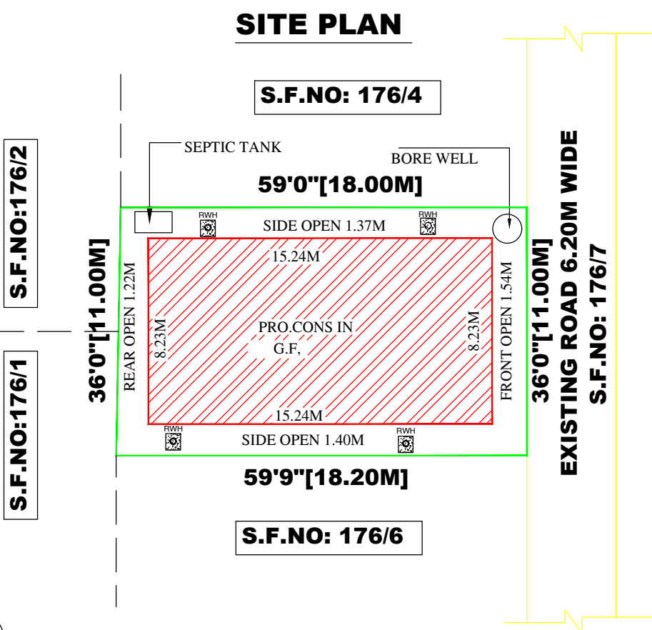
SITE PLAN DETAILS:-
