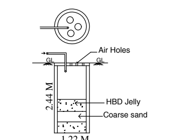
RAIN WATER HARVESTING TANK DETAIL
