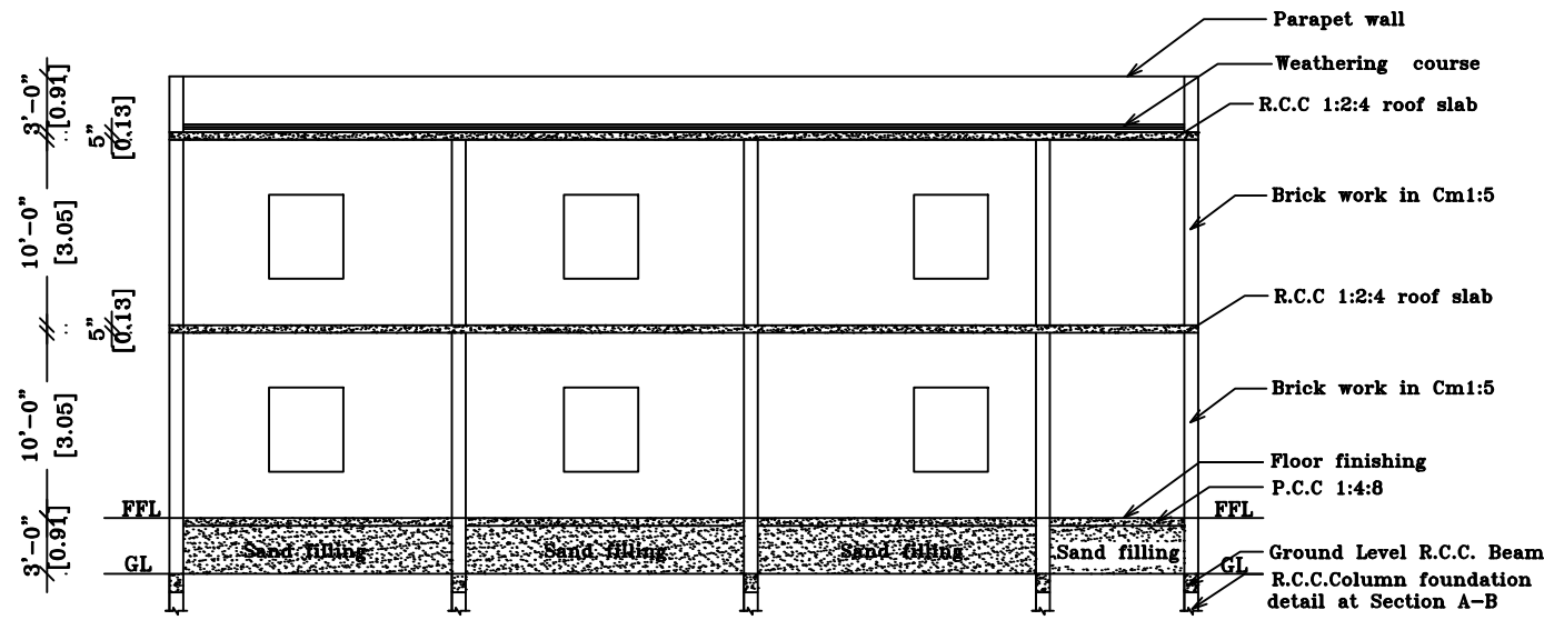
SECTION ON 'SK'
