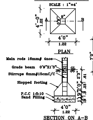
COLUMN DETAILS
