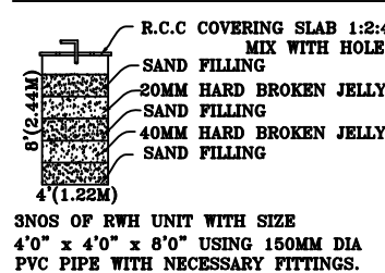
RAIN WATER HARVEST UNIT
