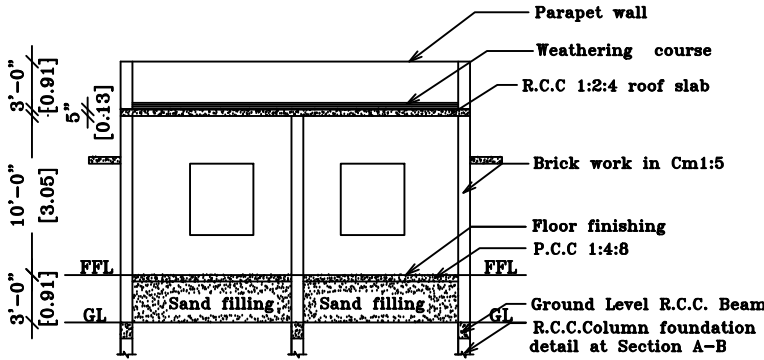
SECTION ON 'SK'
