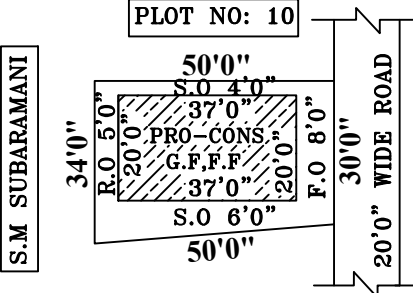
SITE PLAN
