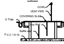
SECTION ON AB1
