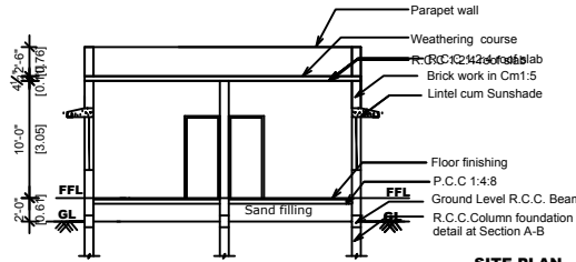
SECTION ON 'RK'
