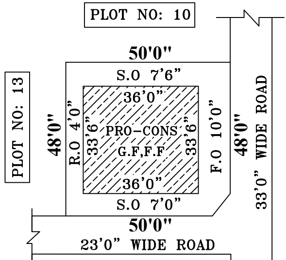
SITE PLAN
