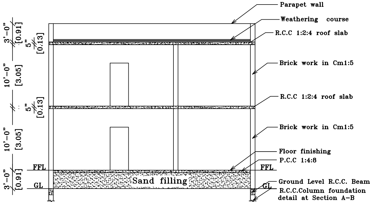
SECTION ON 'SK'
