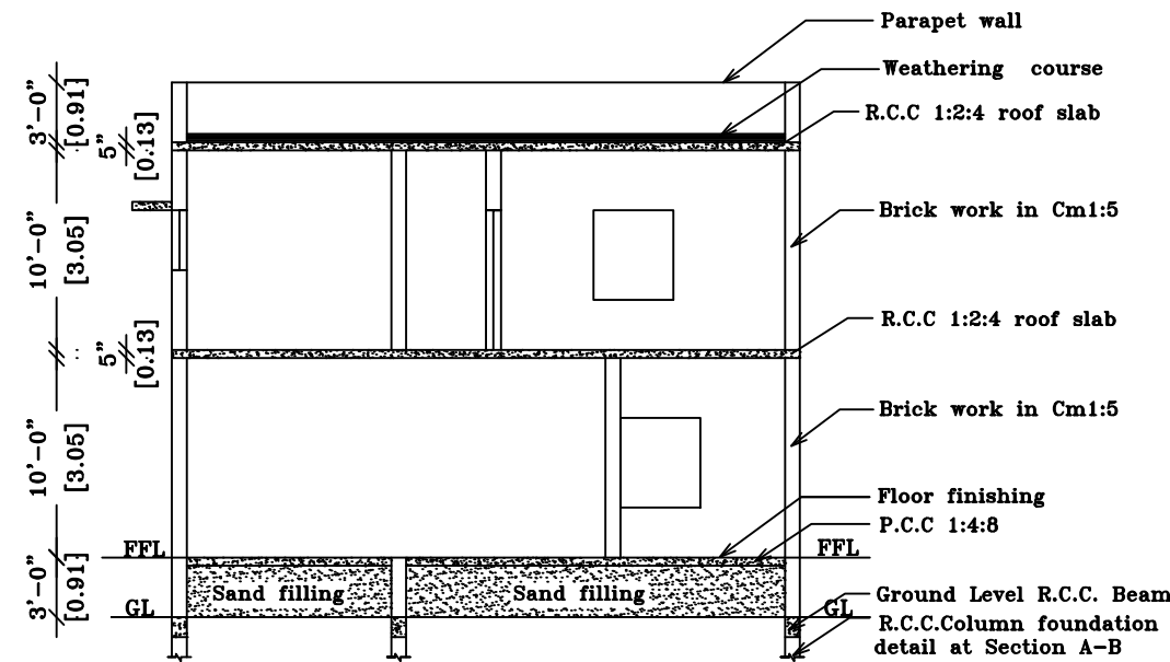
SECTION ON 'SA'
