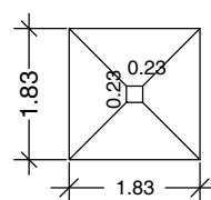
FOOTING
