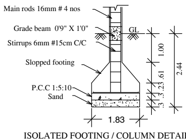
COLUMN DETAIL
