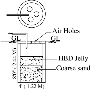
RAIN WATER HARVESTING TANK DETAIL
