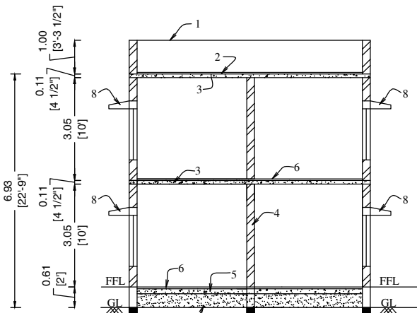
SECTION ON 'JS'
