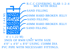
Rain Water Harvesting unit
