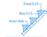
Section of the Staircase Not to scale
