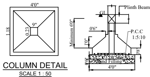
COLUMN DETAIL
