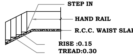
STAIR DETAILS
