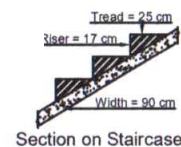
Section on Staircase
