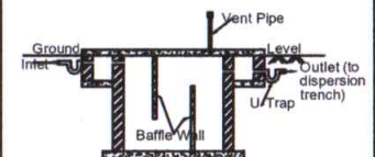
Section on Septic Tank
