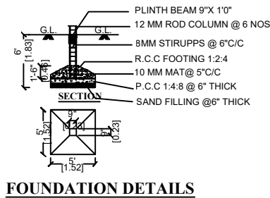
FOUNDATION DETAILS
