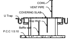
SECTION ON AB1
