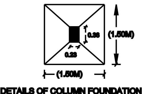
DETAILS OF COLUMN FOUNDATION
