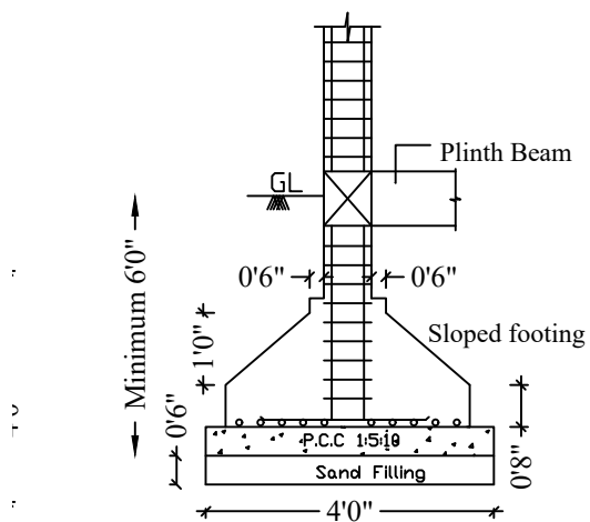
ISOLATED FOOTING / COLUMN DETAIL
