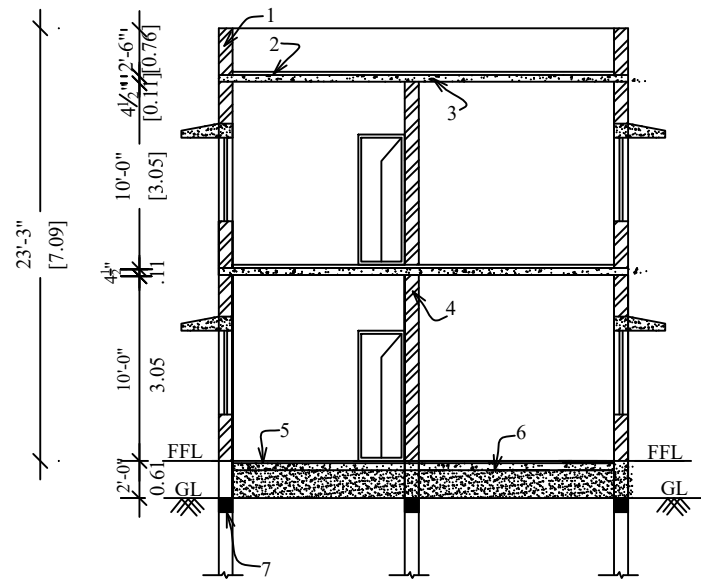
FOUNDATION DETAIL DESIGNED AS PER LOCAL SOIL CONDITION SECTION ON "AB"
