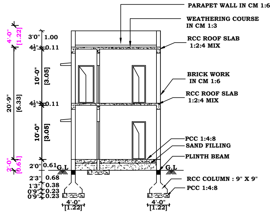
SECTION - KK
