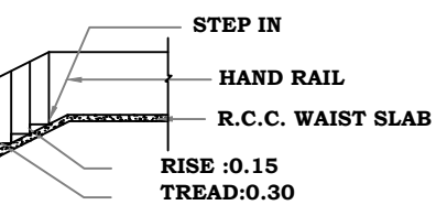
STAIR DETAILS
