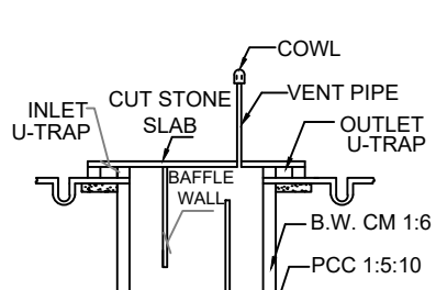
SEPTIC TANK DETAILS SIZE: 6'0" x 3'0" x 6'0"
