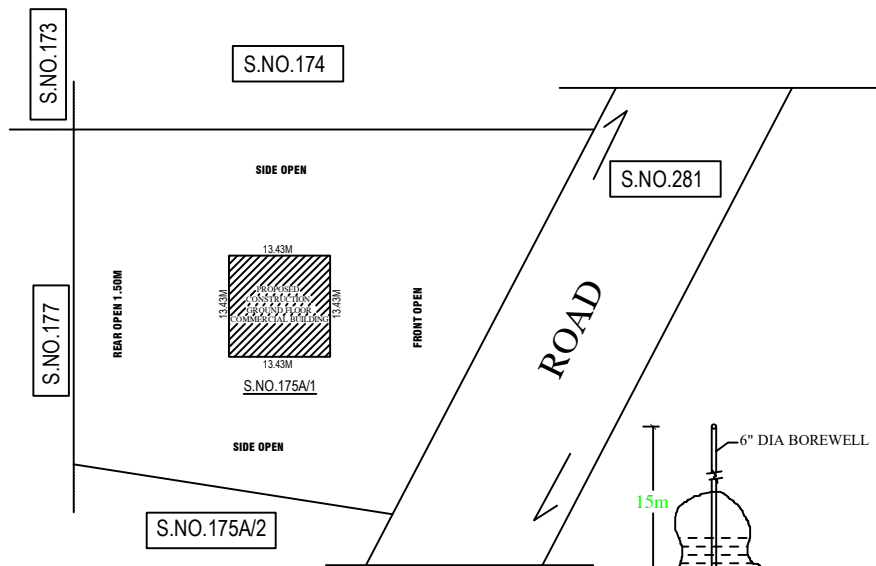
SITE PLAN
