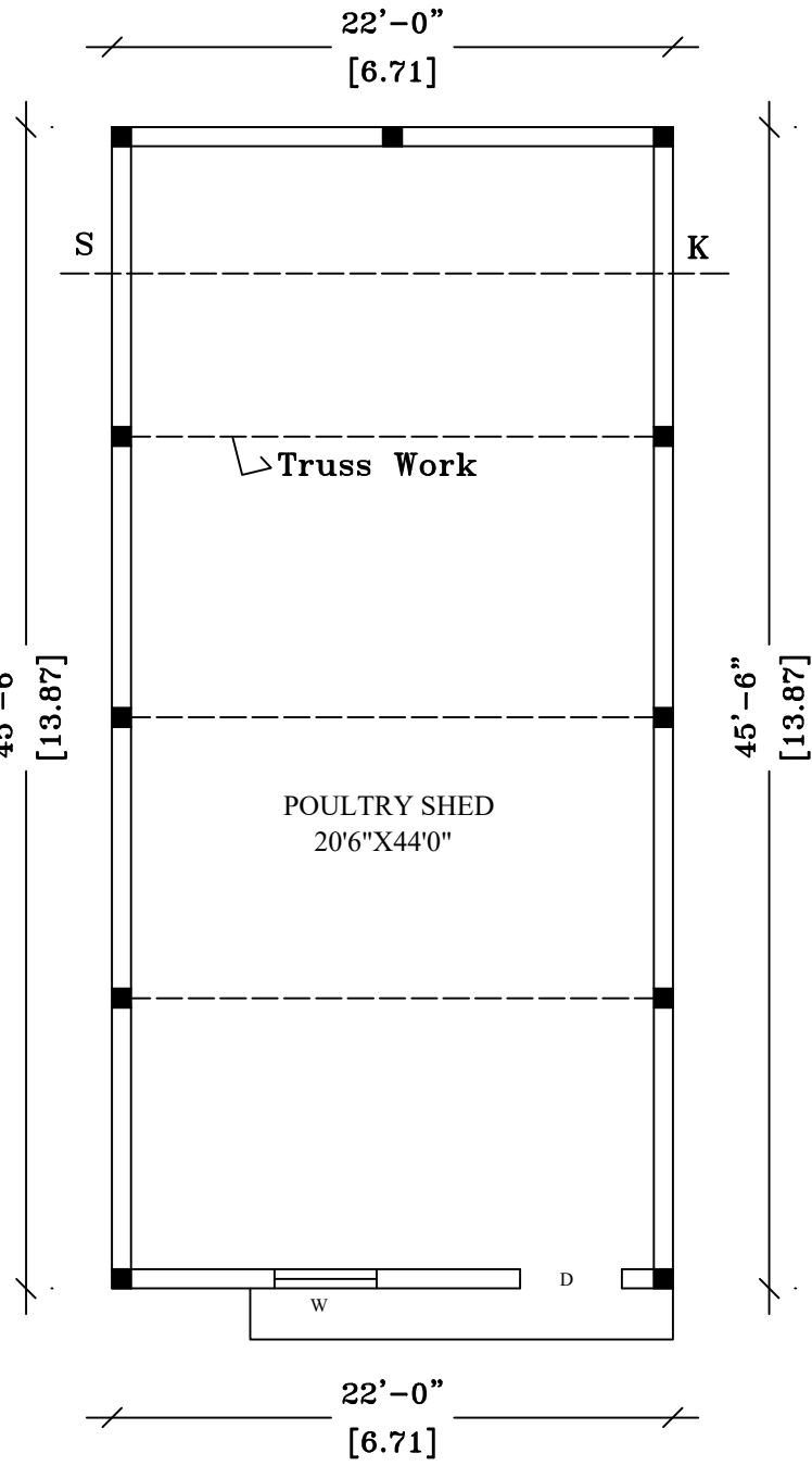
POULTRY SHED
