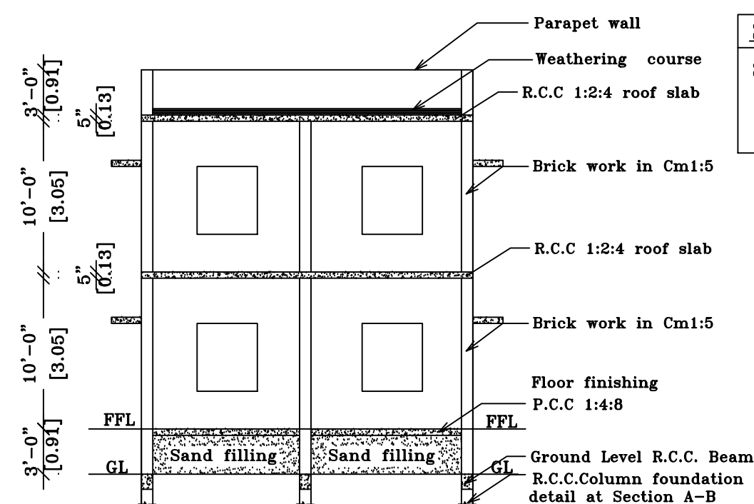
SECTION ON 'SA'
