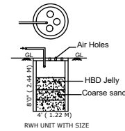
RAIN WATER HARVESTING TANK DETAIL
