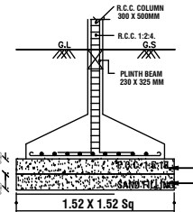
FOUNDATION DETAIL
