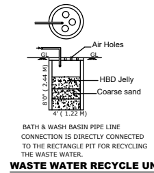
WASTE WATER RECYCLE UNIT
