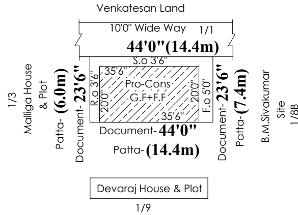
SITE PLAN
