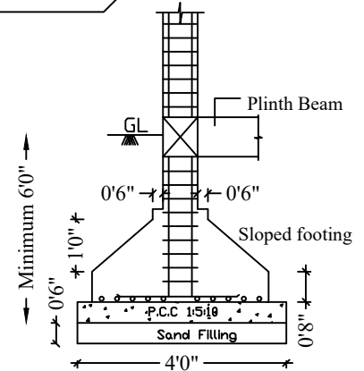
ISOLATED FOOTING / COLUMN DETAIL
