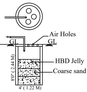
WASTE WATER RECYCLE UNIT
