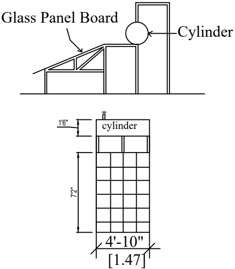
SOLAR ENERGY SYSTEM
