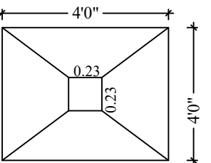
FOOTING / COLUMN DETAIL
