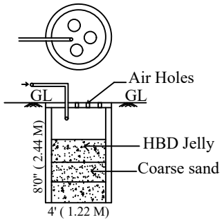
RAIN WATER HARVESTING TANK DETAIL
