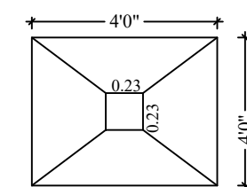
FOOTING / COLUMN DETAIL
