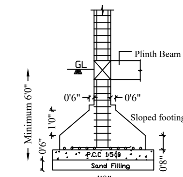
ISOLATED FOOTING / COLUMN DETAIL
