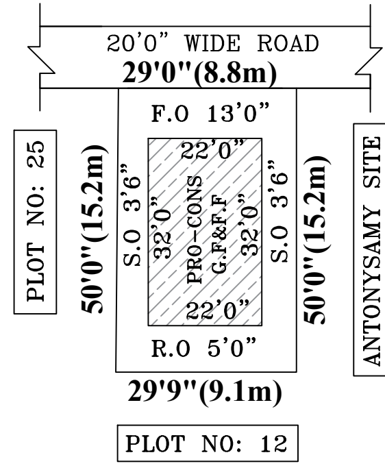
SITE PLAN
