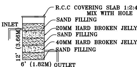
WASTE WATER RECYCLE UNIT
