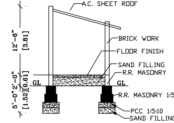
SECTION ON AT 'SK'
