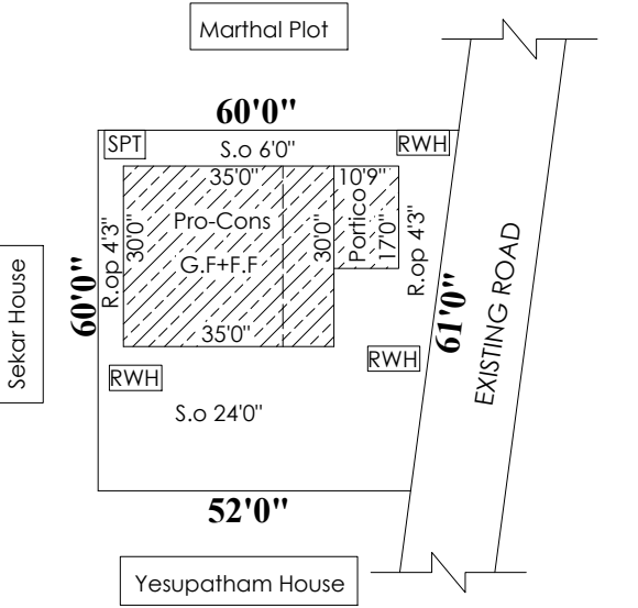
SITE PLAN SCALE:1INCH = 33FEET
