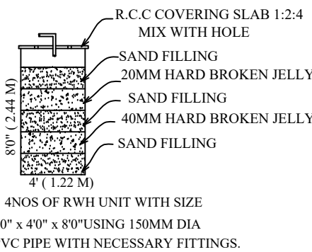
RAIN WATER HARVEST UNIT
