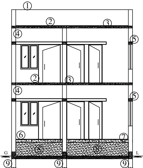
SECTION ON 'CY'
