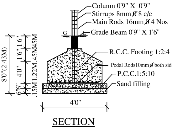
SECTION
