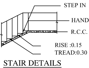
STAIR DETAILS
