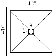
PLAN COLUMN DETAILS SCALE: NOT TO SCALE
