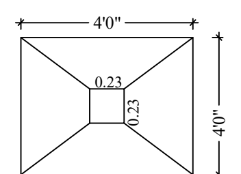
FOOTING / COLUMN DETAIL
