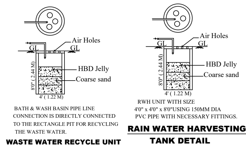
WASTE WATER RECYCLE UNIT
