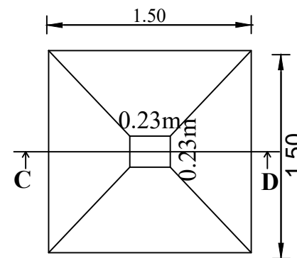
SECTION - 'CD'
