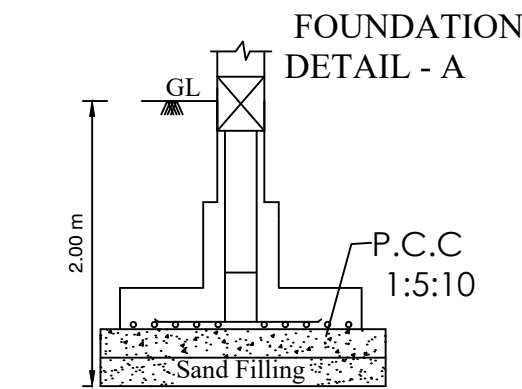
Isolated Footing - A (1.50X1.50) (Not to Scale)
