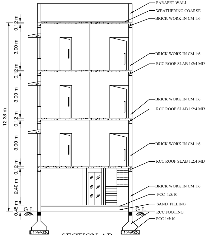
SECTION-AB
