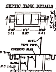
SEPTIC TANK DETAILS
