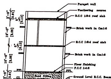
SECTION ON 'SK'
