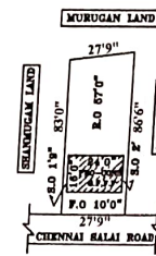
SITE PLAN
