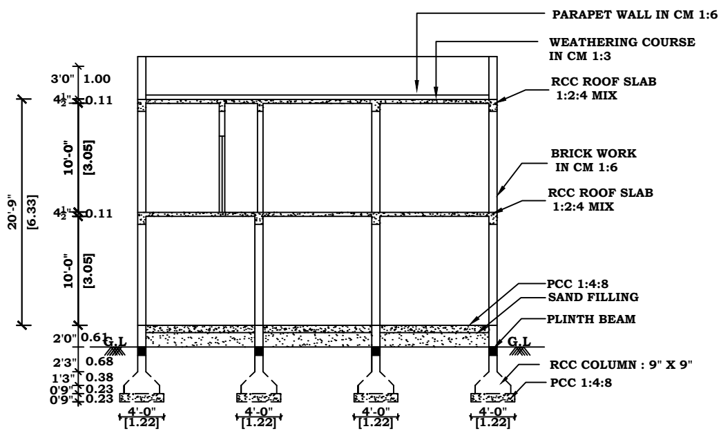
SECTION - KK
