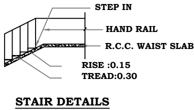
STAIR DETAILS
