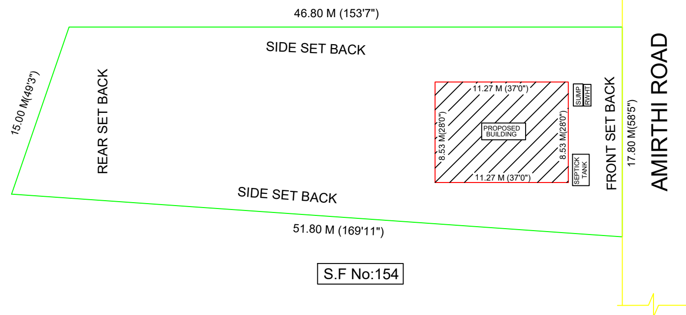
SITE PLAN TO SCALE
