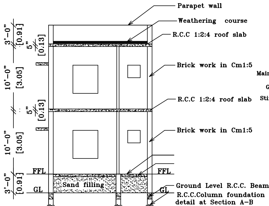
SECTION ON 'SA'
