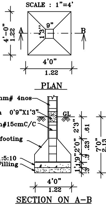
COLUMN DETAILS
