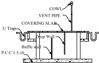
SECTION ON JS1
