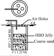
RAIN WATER HARVESTING TANK DETAIL
