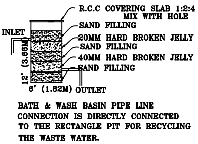
WASTE WATER RECYCLE UNIT
