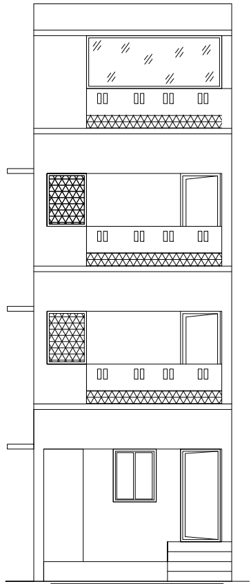
FRONT ELEVATION
