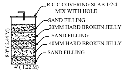
RAIN WATER HARVEST UNIT
