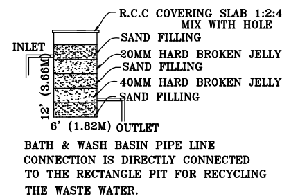
WASTE WATER RECYCLE UNIT
