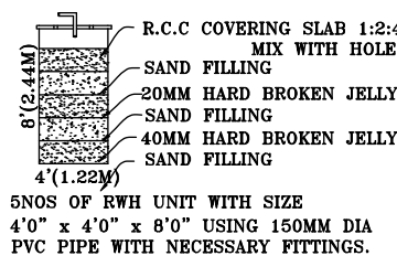
RAIN WATER HARVEST UNIT
