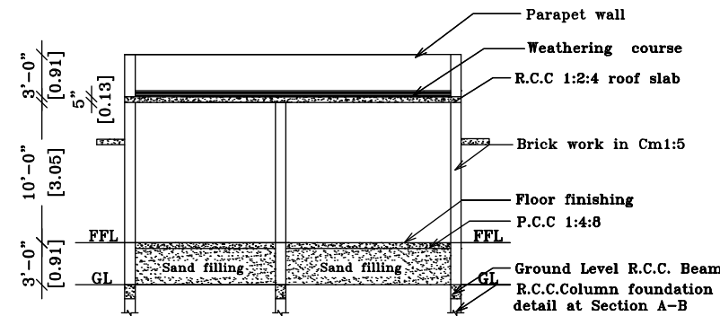
SECTION ON 'SK'
