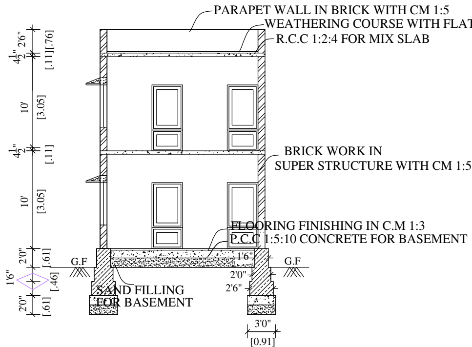
SECTION NO R-S
