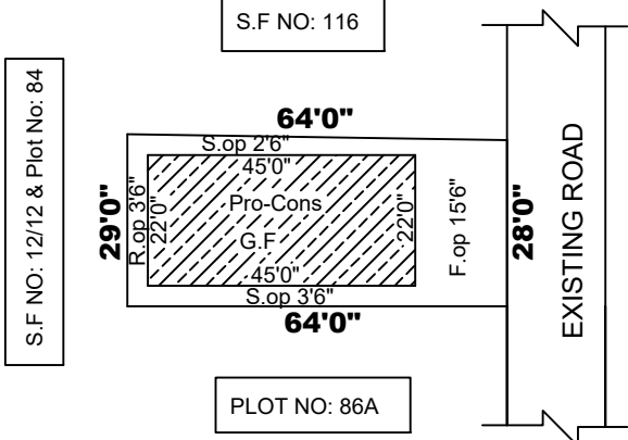
SITE PLAN 1CM=4M
