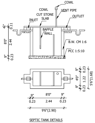
SEPTIC TANK DETAILS
