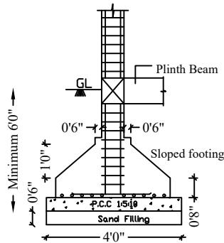
ISOLATED FOOTING / COLUMN DETAIL
