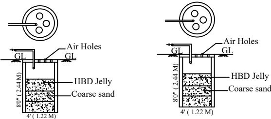
RAIN WATER HARVESTING TANK DETAIL
