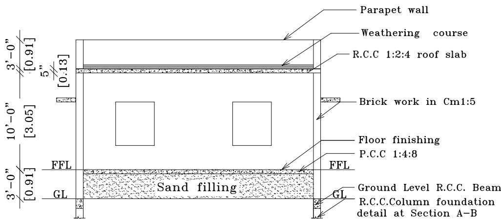
SECTION ON 'SK'
