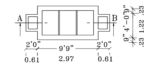
SEPTIC TANK DETAILS
