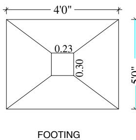
FOOTING
