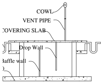
WASTE WATER RECYCLE UNIT
