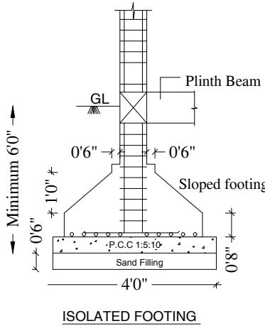
COLUMN DETAILS
